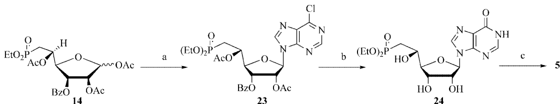
Scheme 4. Preparation of inosine analogue 5 . a) 6-Chloropurine, \text{HMDS} , (\text{NH}_4)_2\text{SO}_4 , reflux then \text{SnCl}_4 ; b) 2-mercaptoethanol, \text{NaOMe} , \text{MeOH} , reflux; c) \text{TMSBr} , \text{DMF} , then TEAB (1 M, pH 7).
