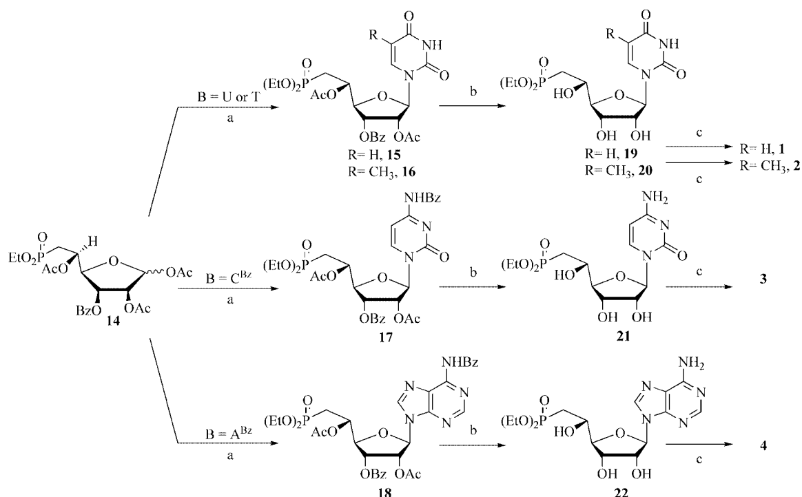
Scheme 3. Synthesis of \beta -hydroxyphosphonate nucleoside analogues, 1–4 . a) Nucleic base ( \text{B} = \text{U} or \text{T} or N^4 -benzoylcytosine or N^6 -benzoyladenine), BSA, \text{CH}_3\text{CN} , reflux then \text{SnCl}_4 ; b) \text{NH}_3 , \text{MeOH} ; c) \text{TMSBr} , \text{DMF} , then water or TEAB (1 M, pH 7).
